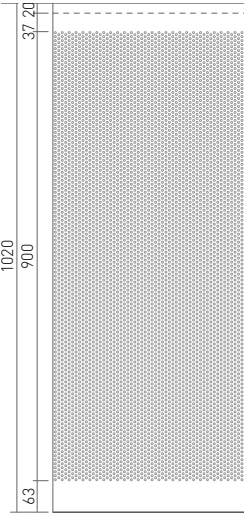
Fig B1.4: Trimoterm Sound RV Ø4 x 8 perforation
